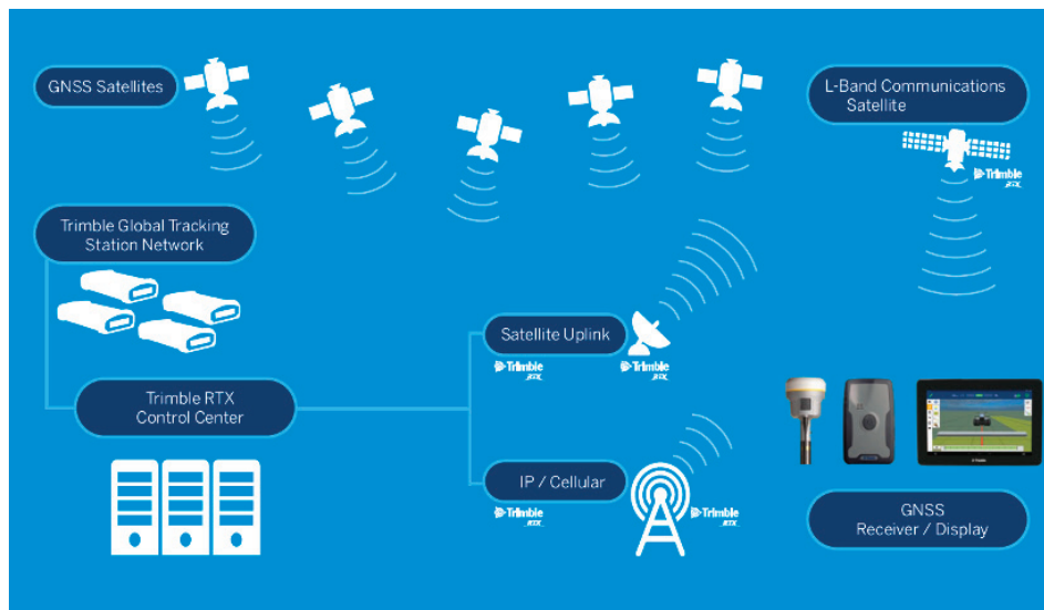
How Trimble CenterPoint RTX works
